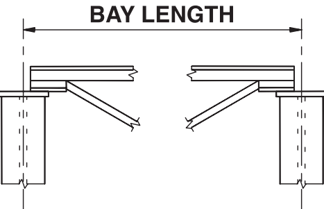
STEEL COLUMN
