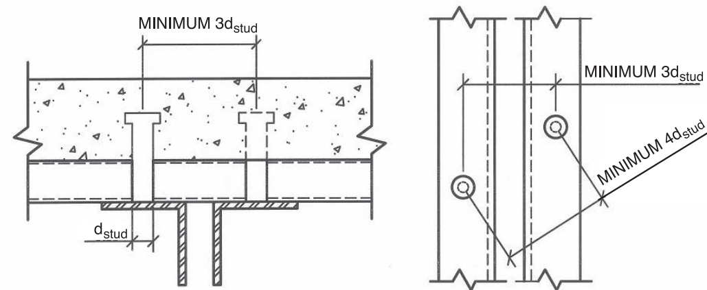
FIG. 12 - MINIMUM TRANSVERSE SHEAR STUD SPACING THE STUDS SHALL BE TRANSVERSELY SPACED A MINIMUM OF 3 STUD DIAMETERS WHEN SHEAR STUDS ARE STAGGERED WITHIN ONE DECK RIB.
