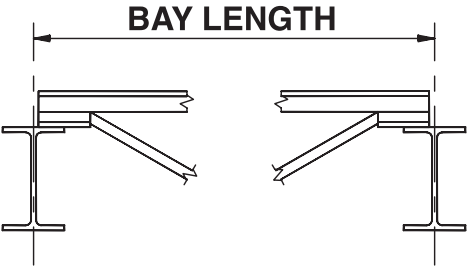
STEEL BEAM
