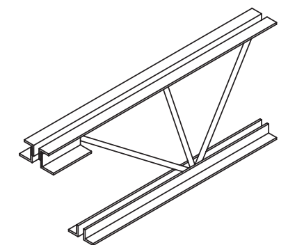
FIG. 3 - BOTTOM CHORD EXTENSION
