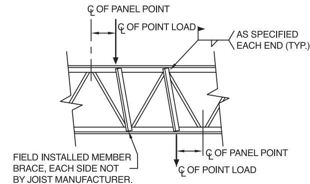
FIG. 1 - TYPICAL JOIST REINFORCEMENT AT CONCENTRATED LOADS
