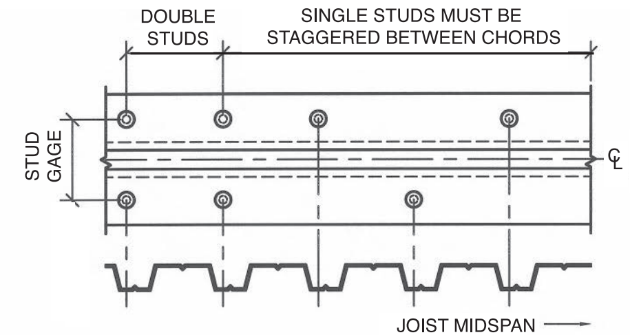
FIG. 14 - SINGLE AND DOUBLE SHEAR STUD POSITIONS ON TOP CHORD
