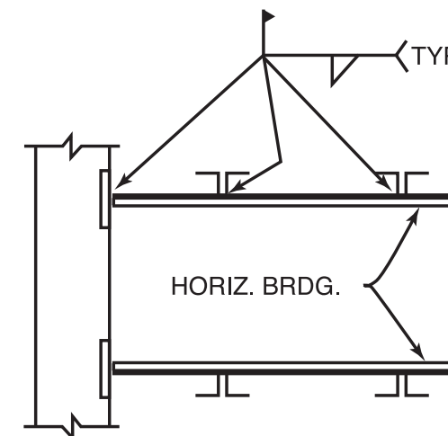
HORIZONTAL BRIDGING TERMINUS AT PANEL WALL
