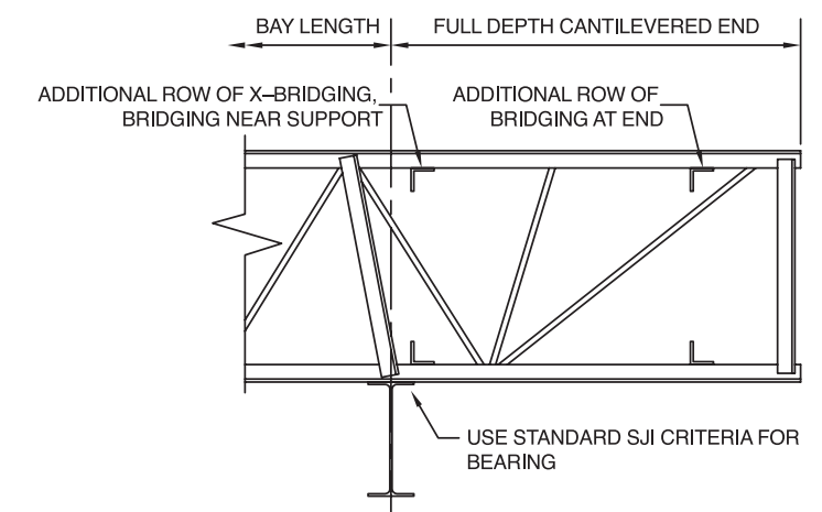
FIG. 5 - CANTILEVERED, BOTTOM BEARING, SQUARE END
